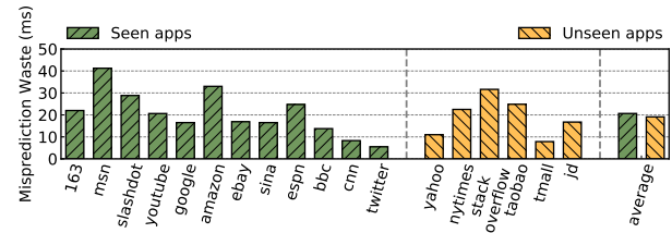
Fig. 10: The average mis-prediction waste.
