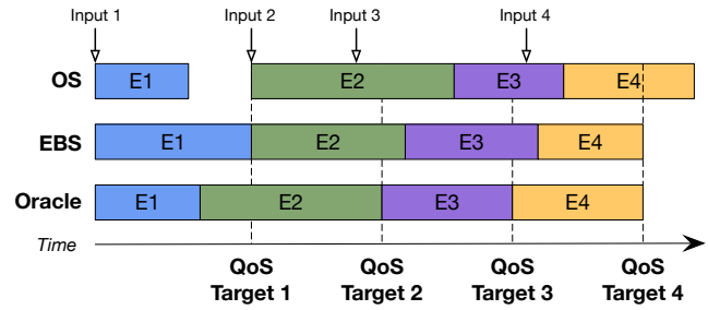
Fig. 2: Comparison of different scheduling mechanisms using a representative interaction sequence from cnn.com . Each input (top of the figure) triggers an event execution, and corresponds to a particular QoS target (bottom of the figure). OS and EBS are reactive schedulers and lead to QoS violations or energy waste. The oracle scheduler can proactively coordinate executions across events, and thus eliminates all QoS violations and minimizes energy consumption.
