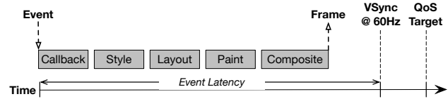
Fig. 1: The user QoS is dictated by the event latency, which, if exceeds the QoS target (deadline), degrades responsiveness.
